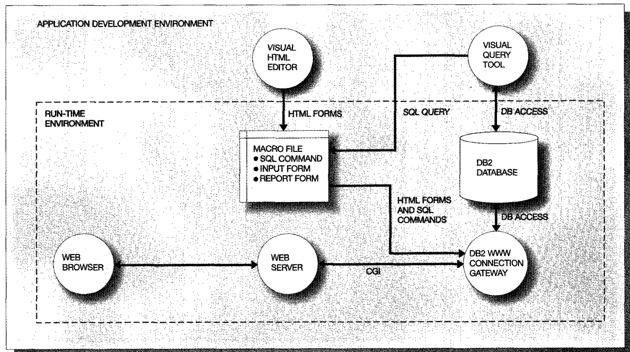
Figure 3 DB2 WWW Connection system overview
