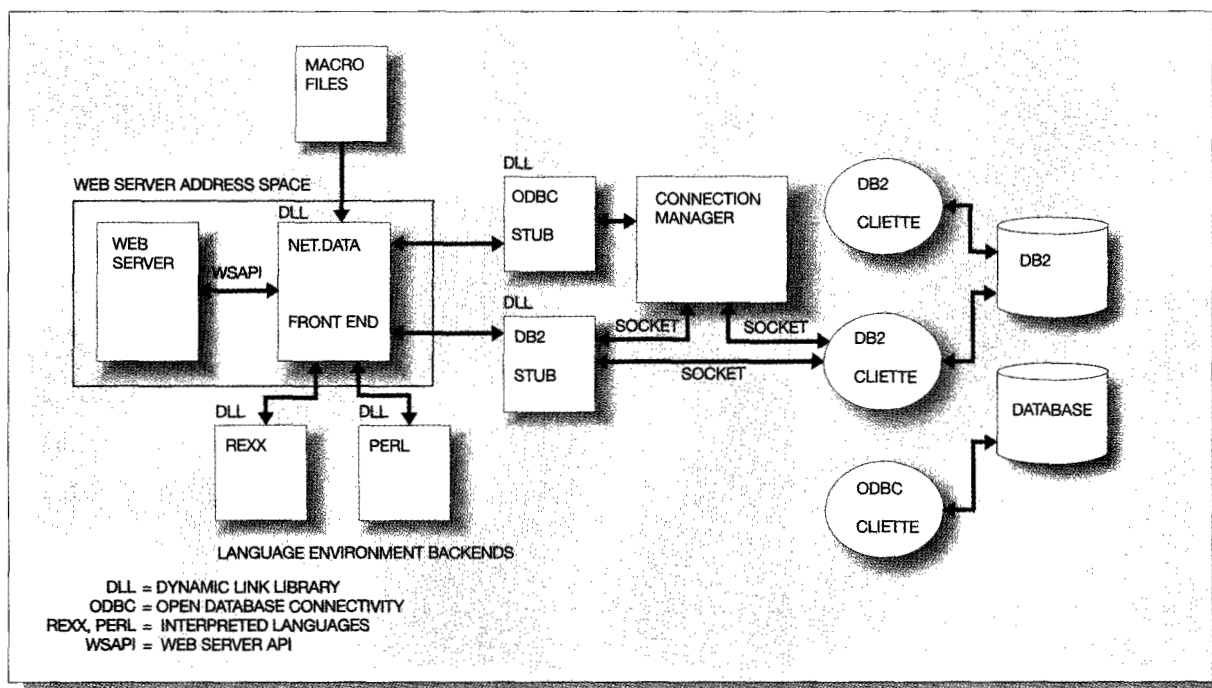
Figure 8 Net.Data overview
