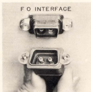
Pluggable connector for Spectronics fiber optic data transmission system.
