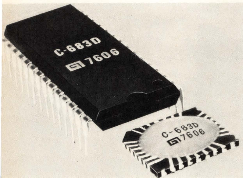
5. Epoxy-glass pack. General Instrument supplies a line of MOS chips in this 1/2-inch-square, low-cost epoxy-glass carrier called a Minipak. On the bottom are solder bumps that can be reflow-soldered to a pc board. A drop of epoxy protects the chip.
