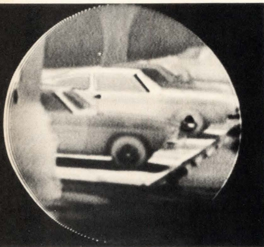
Pretty sharp. Philips' high-resolution room-temperature pyroelectric vidicon yields a picture that is quite detailed for an IR image.
