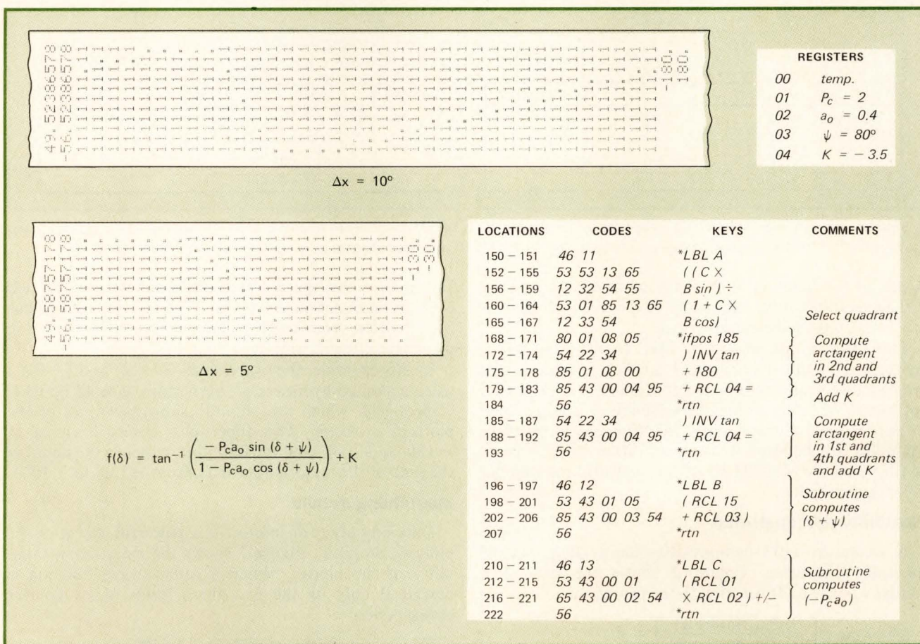
2. Phase-shift function. The SR-52 and printer can easily plot complex functions like this one, which has a shape not clearly described by the equation. Note the use of sub-subroutines in this program. Lower plot is a magnification of upper plot between -130^\circ and -30^\circ .
