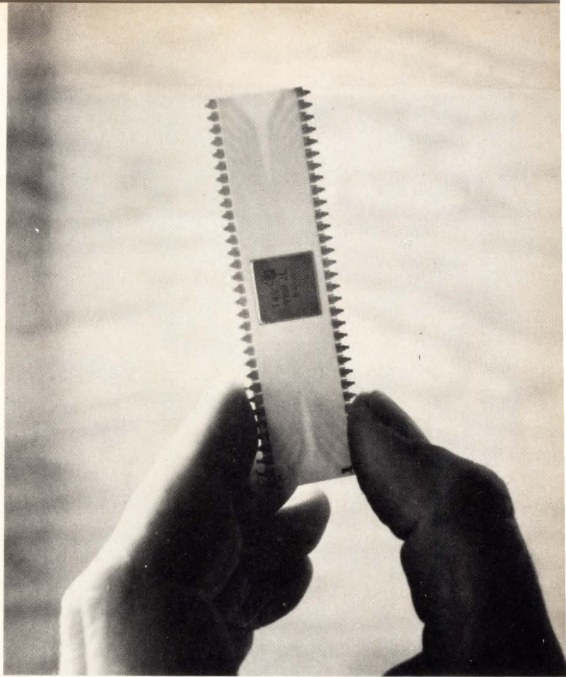
1. Big DIP. The largest commercially available package for LSI chips is this 3.2-by-0.9-inch, 64-lead, cofired ceramic dual in-line package. Packages of this type are only used for complex, expensive LSI circuits like microprocessors and extremely large memories.
