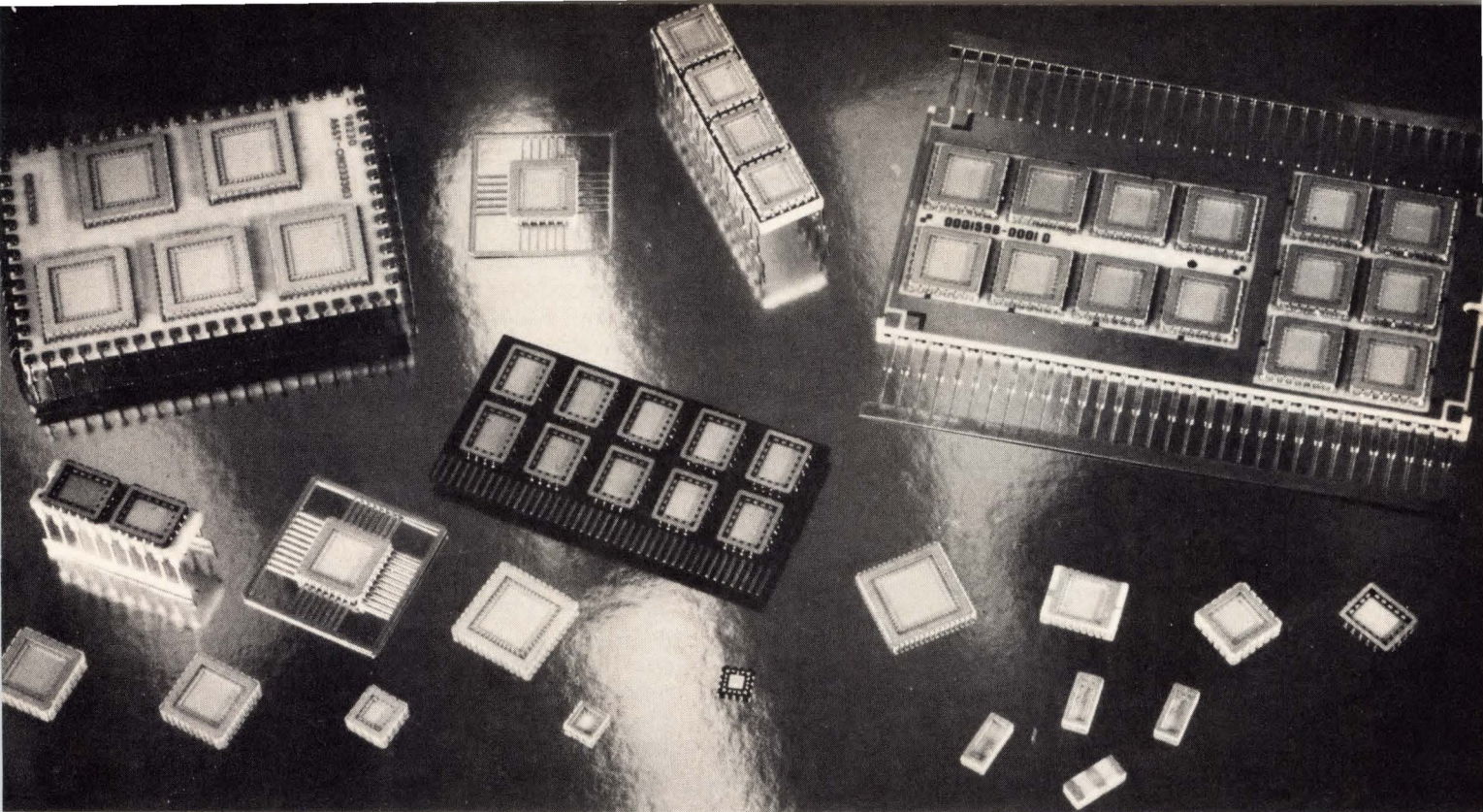
3. Carrying chips. The cofired ceramic chip-carriers shown along the bottom of this view come in a variety of forms—note the leaded chip-carriers in the lower left and upper center. Several large and small ceramic motherboards for the groups of carriers are also shown.
